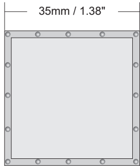
Braille Frame
